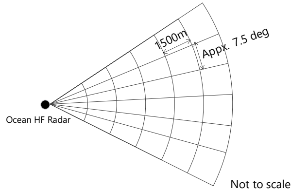
Figure 1 Radar Range-Direction Grids
