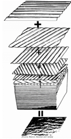
Figure 2 Decomposition of Random Sea Surface Motion[6]
